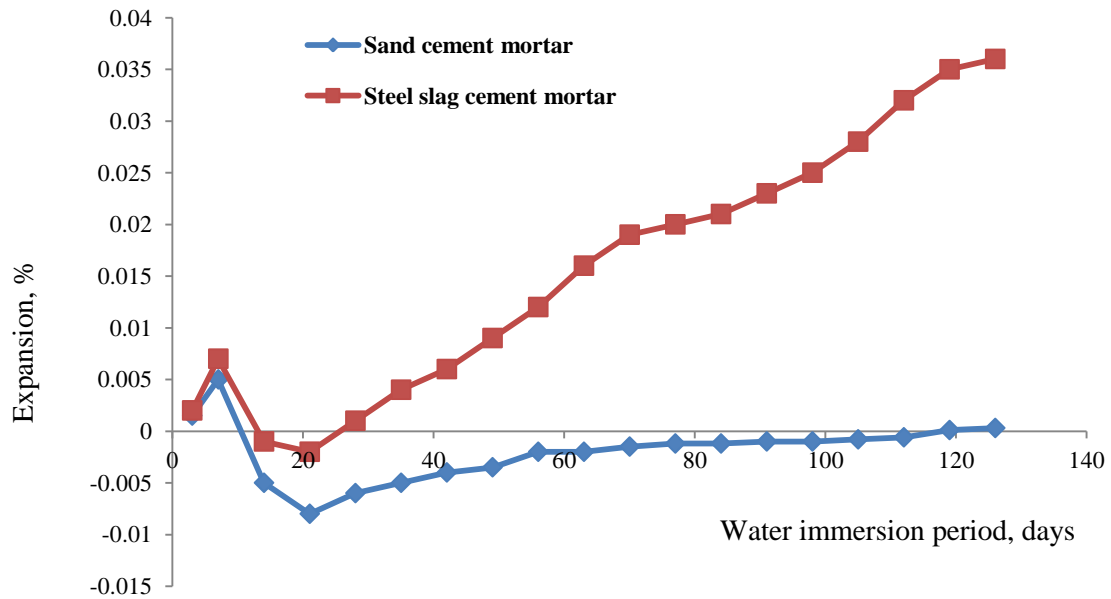
Figure 10. Expansion of the steel slag and sand cement mortars
