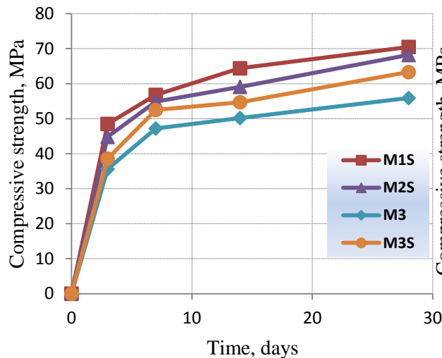
Figure 4. Compressive strength of concrete using basalt and steel slag coarse aggregate at various time
